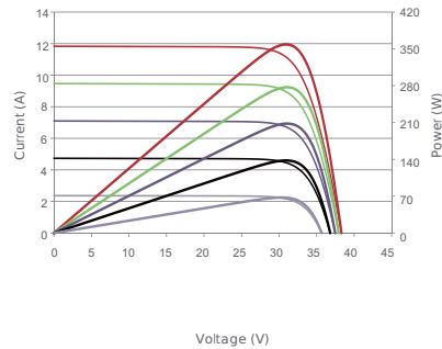
Current-Voltage & Power-Voltage Curves (370W)
